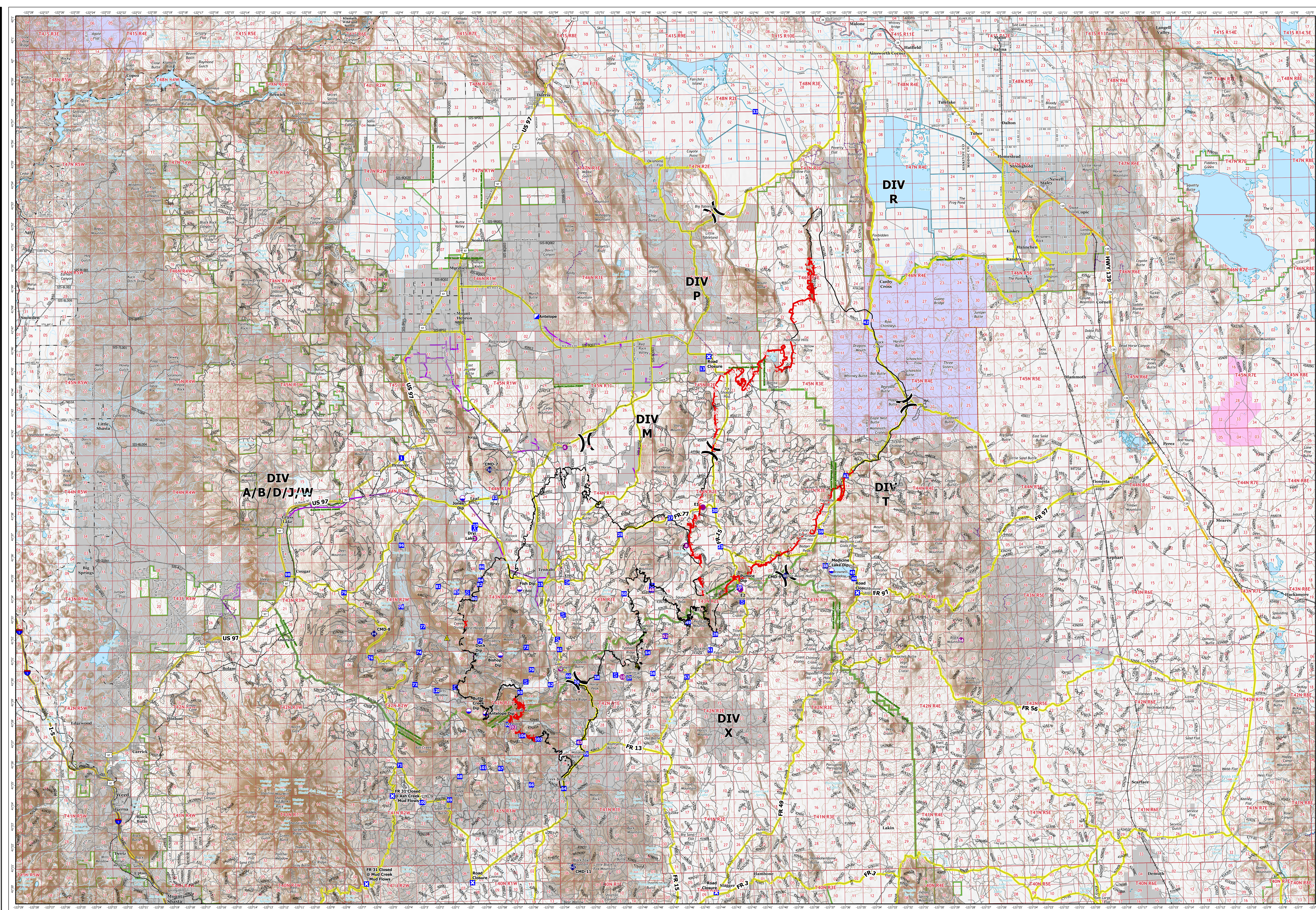
Transportation Map Antelope Fire CA-KNF-006454 9/18/2021 145,188 acres at 9/17/21 2100
