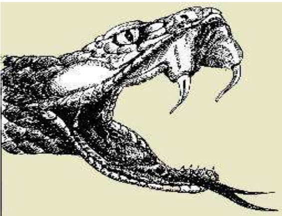
Snake
