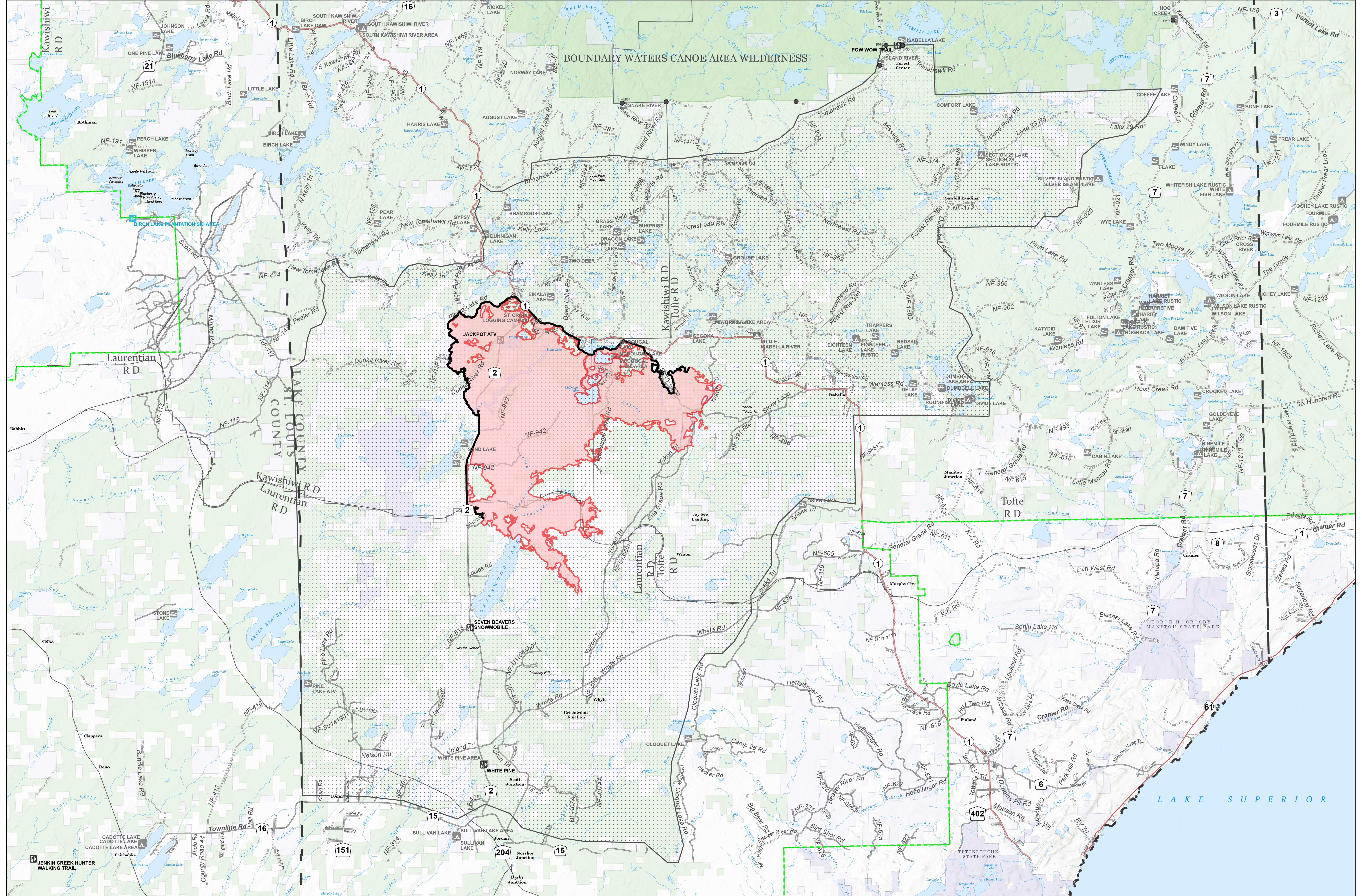
Fire Perimeter as of 09/06/2021 0045 hrs 26,112 Acres
