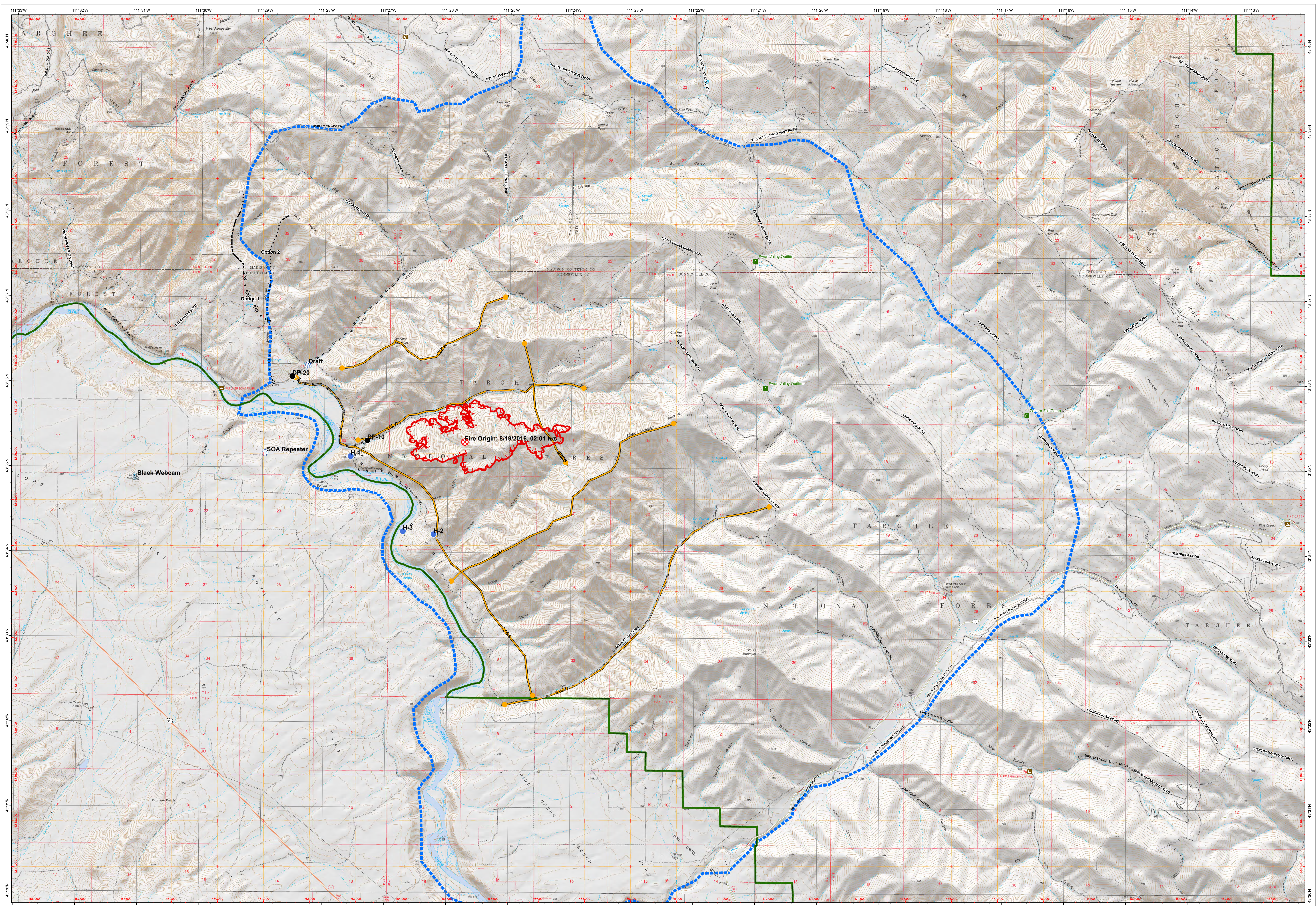
Black Fire Operations Map ID-CTF-003168 Day Operations: 9/9/2016 642 acres as of: 9/7/2016, 22:20 hrs NAD 1983 UTM Zone 12N CMM 20160908
