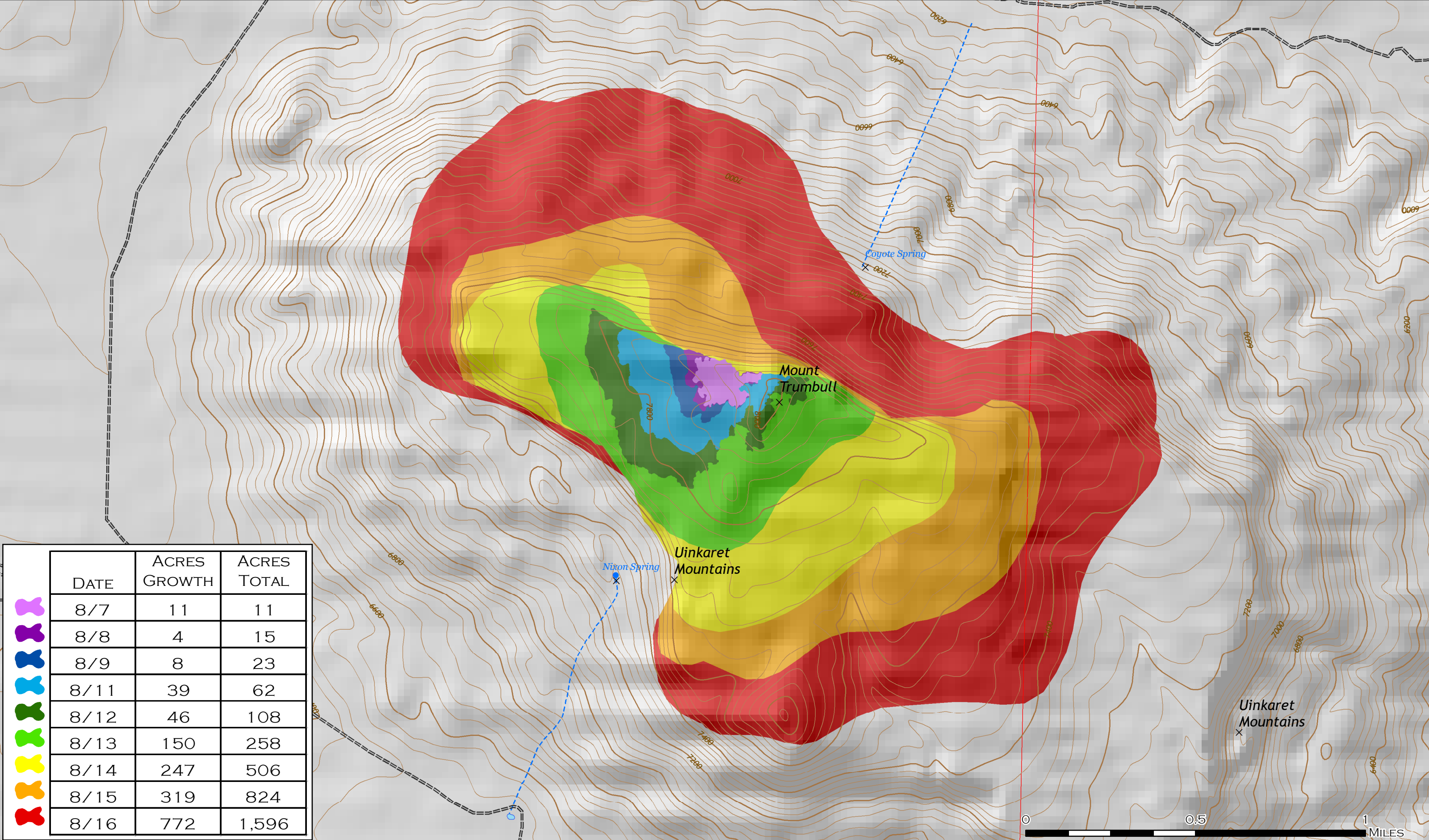
TRUMBULL FIRE PROGRESSION MAP 1,596 ACRES - AUGUST 17, 2019
