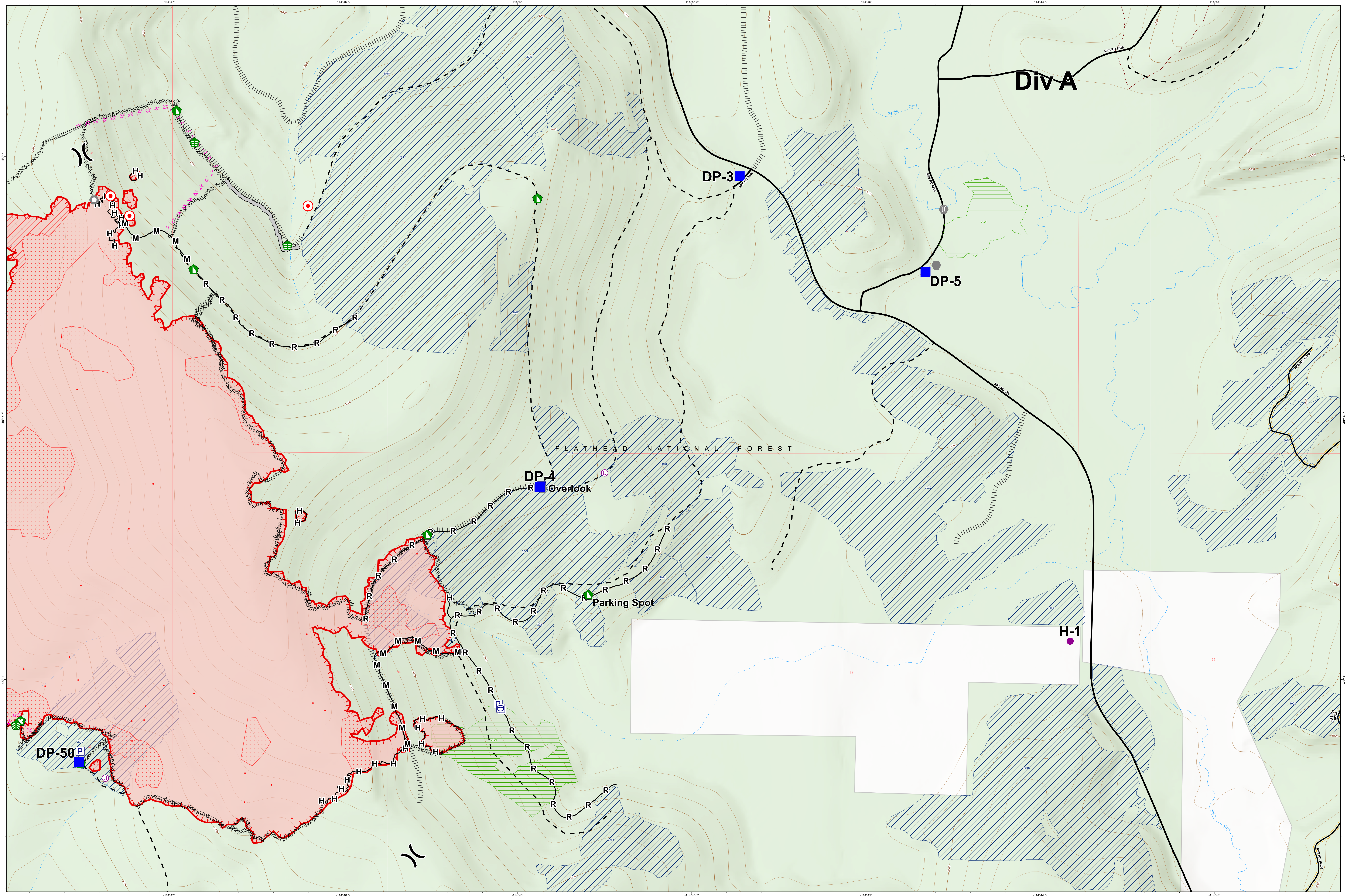
Lemonade MT-FNF-000651 Fire Perimeter as of 09/09/2022 2200 hrs 660 Acres
