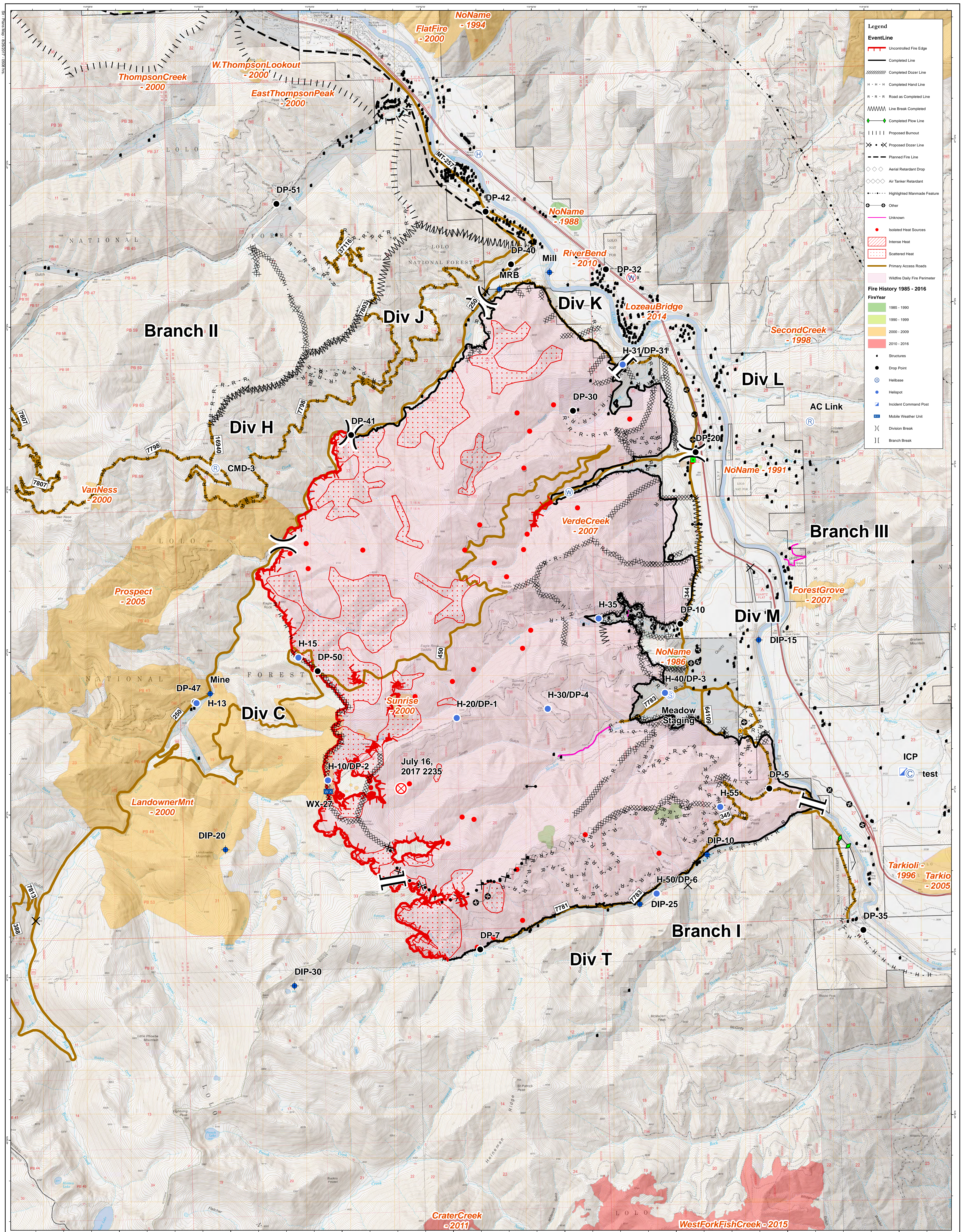
Sunrise Fire - MT-LNF-001336 - Situation Map Perimeter from IR - 8/25/17 - 2126 hrs - 25,600 acres
