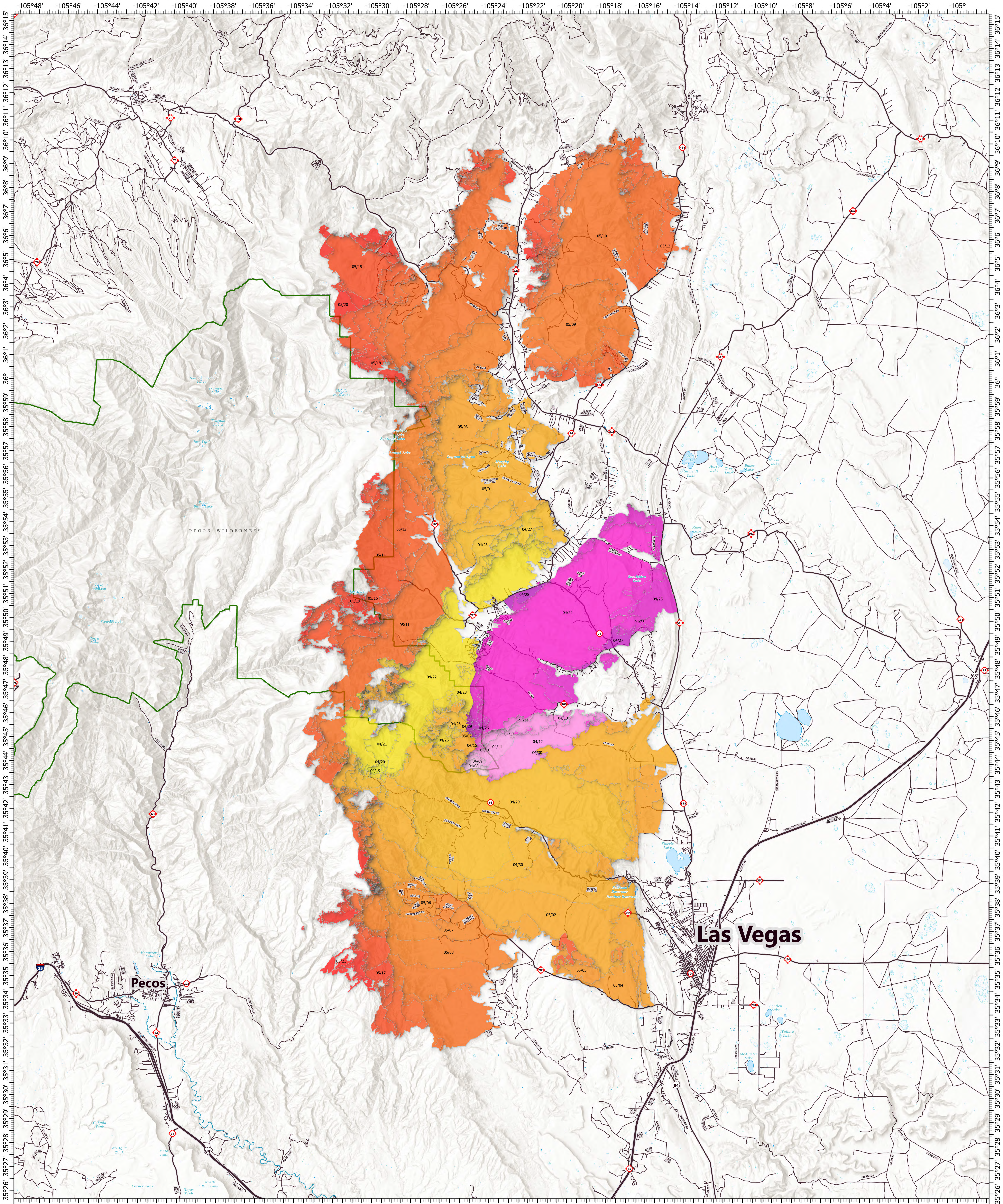
Hermit Peak Fire Progression
