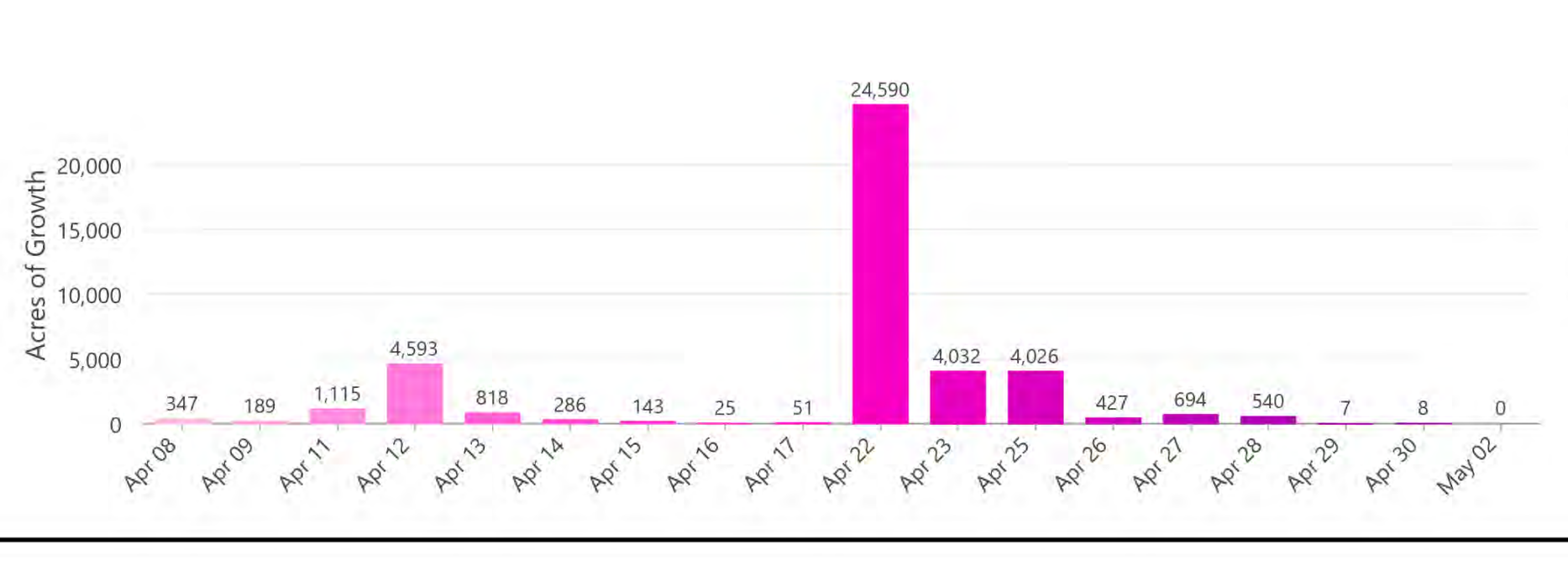
Hermit Peak Fire Progression
