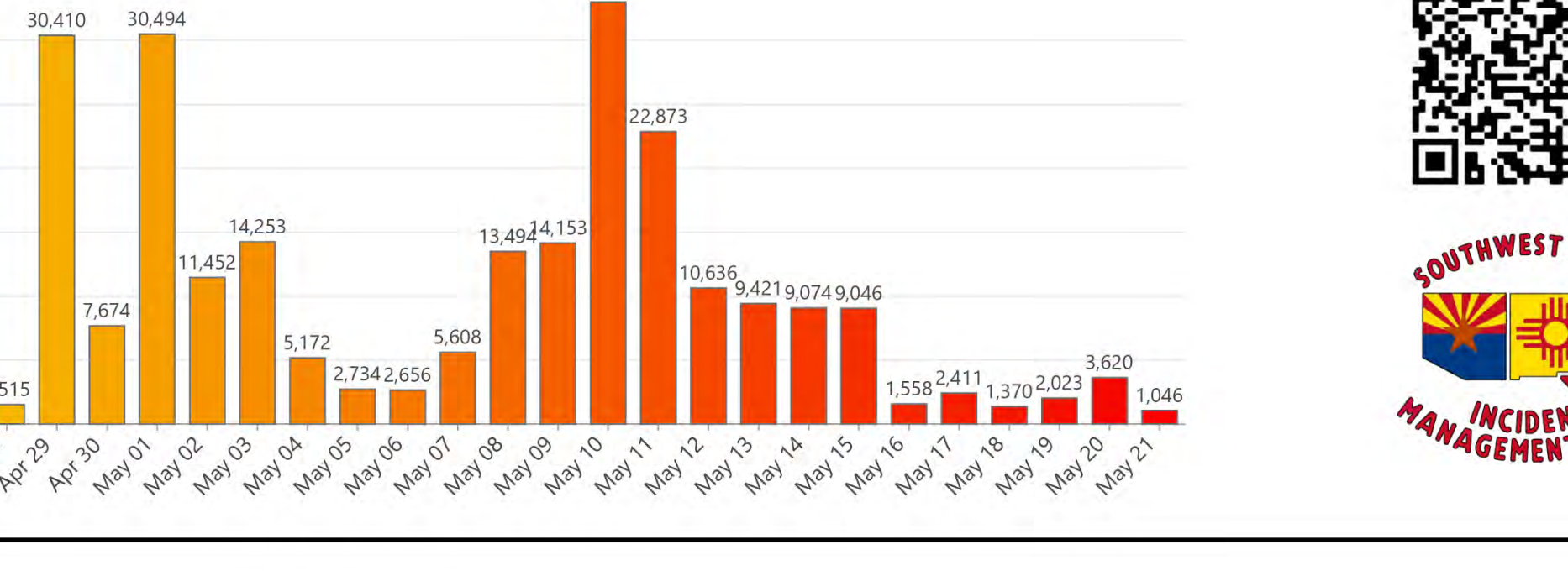
Calf Canyon Fire Progression
